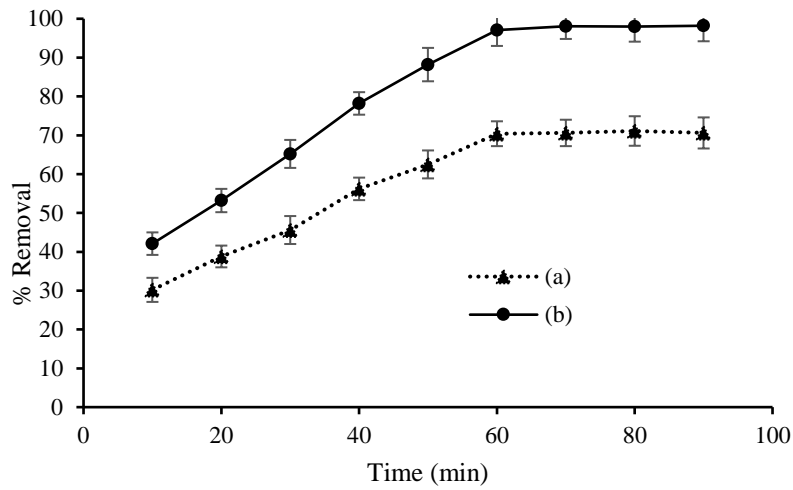
Figure 6. Effect of the contact time on the removal of Pb(II) by (a) Hydroxyapatite and (b) Hydroxyapatite-SiO 2 composite
