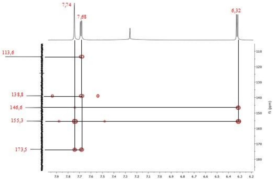
Figure 7. HMBC spectrum of 2,5-dihydroxyphenylethanone
