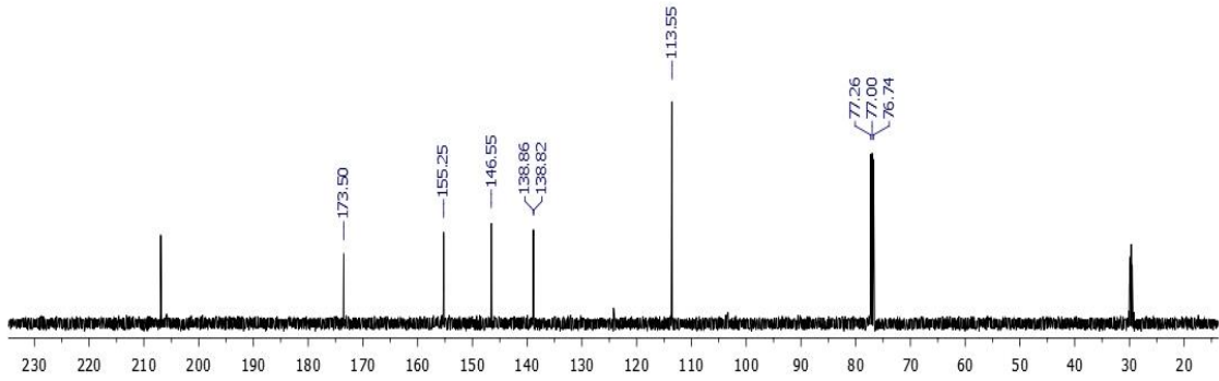
Figure 5. 13 C NMR spectrum of 2,5-dihydroxyphenylethanone
