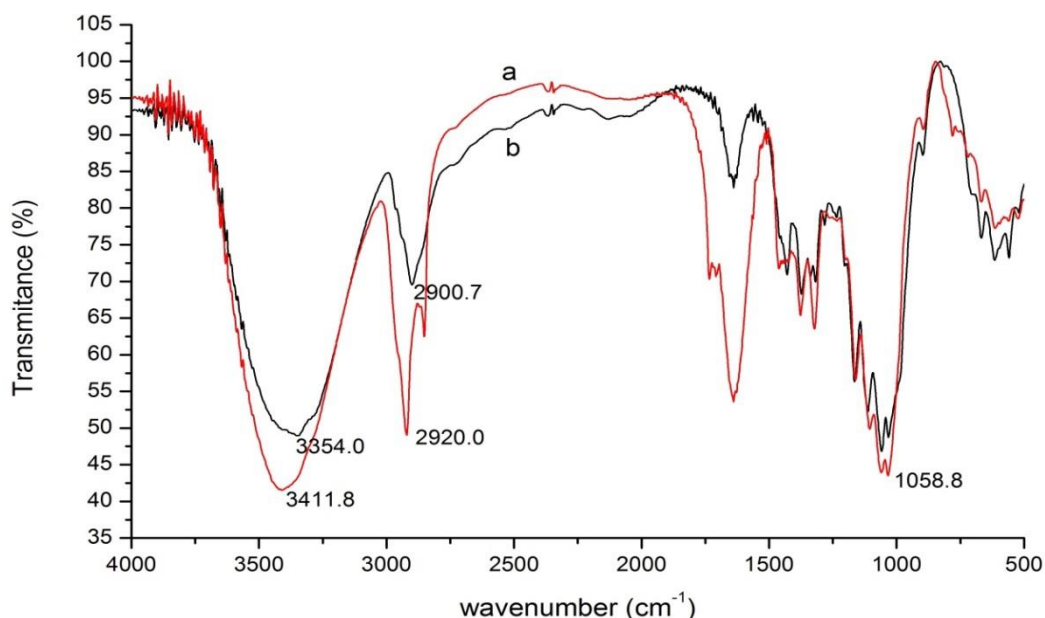
Figure 1. FTIR Spectra of (a) cellulose extracted from kepok banana peel and (b) standard of cellulose
